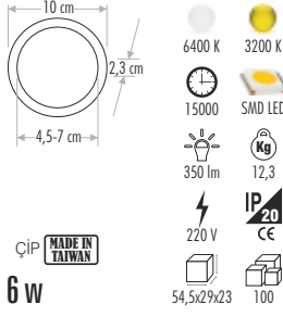
CT-5645 PLUS LED PANEL ARMATÜR 25,00 ₺
