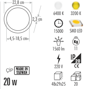
CT-5648 PLUS LED PANEL ARMATÜR 60,00 ₺
