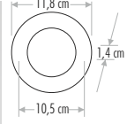
CT-5145 3" PANEL LED ARMATÜR 22,00 ₺
