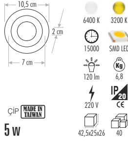
CT-5120 OKYANUS LED PANEL ARMATÜR 35,00 ₺
